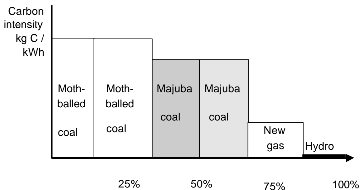
Figure 2: Near future reference scenario carbon intensity (kg CO 2 /kWh) against the share of generation (TWh)
