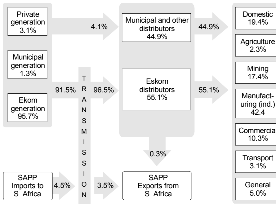
Figure 2: Energy flow through the electricity supply industry in South Africa 3
