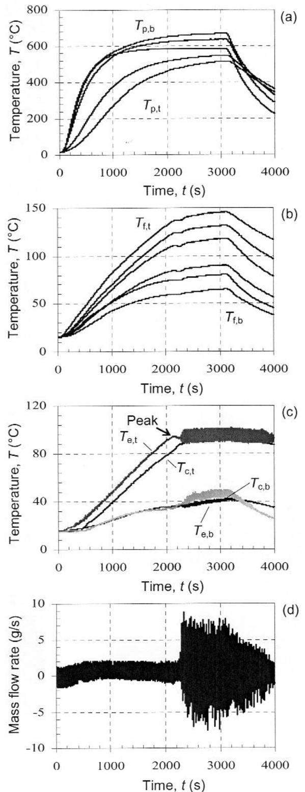
Figure 3. (a) Heating plate temperatures (b) Fin temperatures, (c) Working fluid temperatures (d) Mass flow rate.
