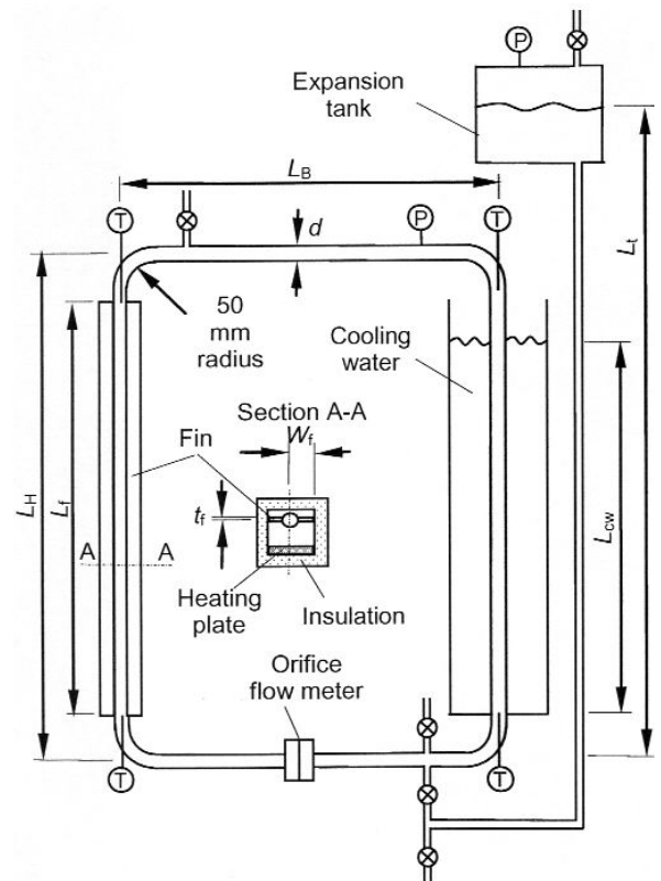
Figure 2: Schematic representation of a natural circulation experimental loop showing important dimensions
