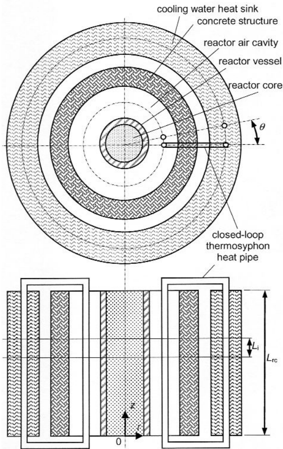
Figure 1: Schematic representation of the axially symmetrical RCCS showing equally spaced closed loop thermosyphon heat pipes spaced around the periphery of the reactor at a pitch angle \theta
