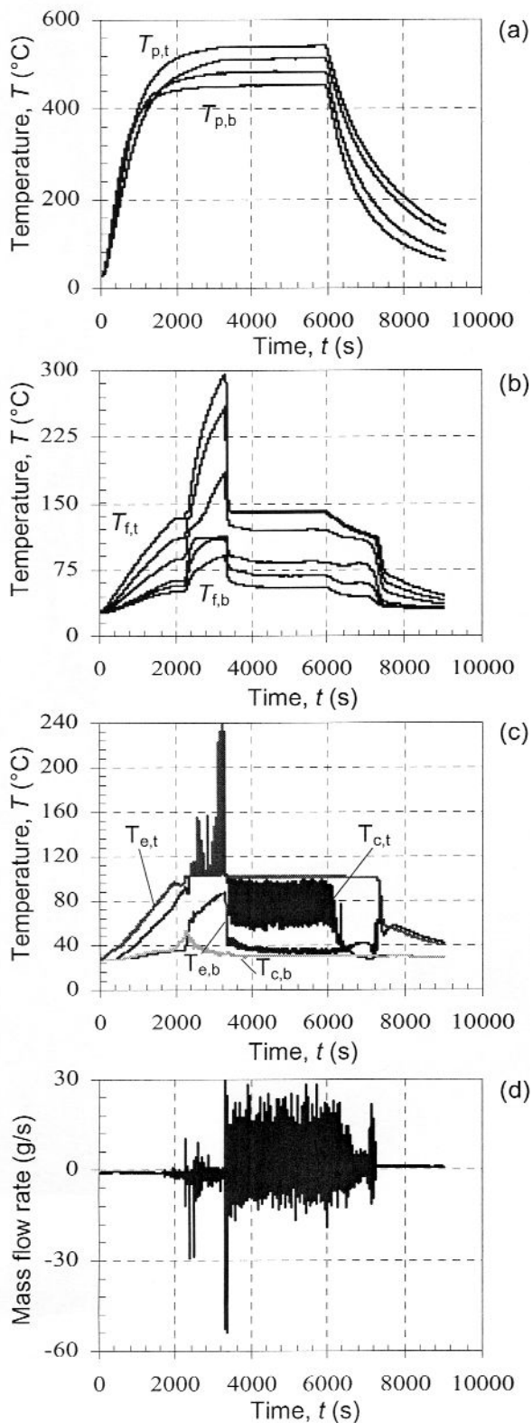
Figure 4: (a) Heating plate temperatures (b) Fin temperatures (c) Working fluid temperatures (d) Mass flow rate
