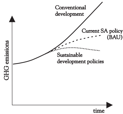
Figure 3.2. Theoretical Impact of Current South Africa Policy on Trajectory of Greenhouse Gas Emissions Relative to Conventional and Sustainable Development Paths
