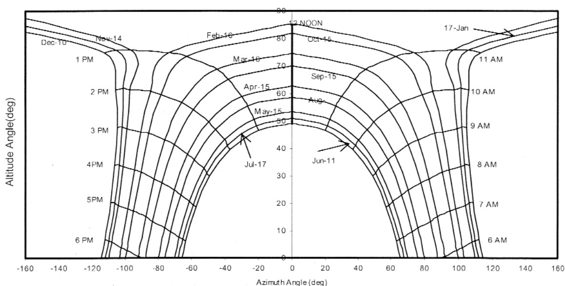
Figure 1: Sun chart for Harare, latitude 17.8°S
