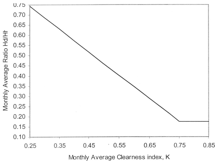
Figure 7: Correlation of the monthly average daily diffuse ratio with monthly average clearness index for Zimbabwe
