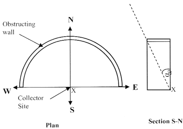
Figure A1: Plan and section of collector site
