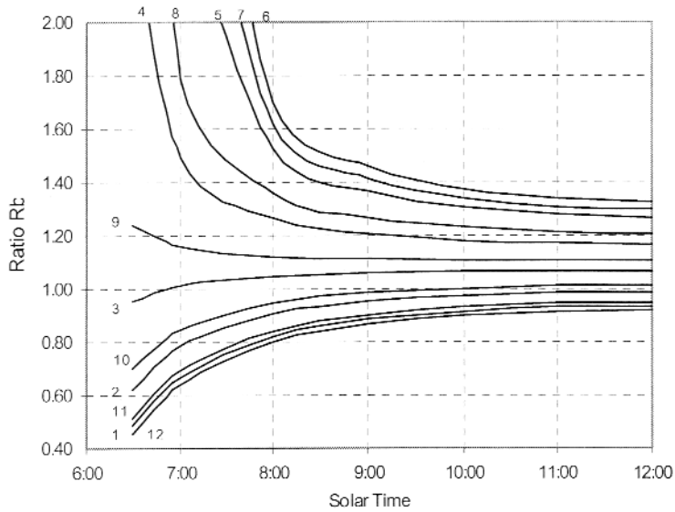
Figure 4b: Ratio R_b for latitude 23^\circ\text{S} for a north-facing collector with tilt angle equal to latitude
