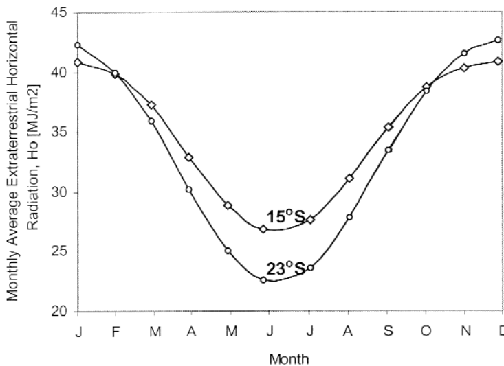
Figure 6: Monthly average daily extraterrestrial irradiation on a horizontal plane for latitudes 15 and 23°S
