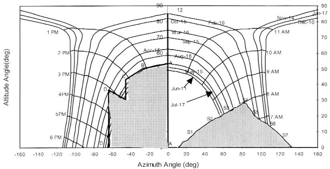
Figure 3: Shading mask superimposed on sun chart
