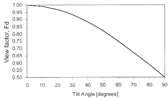
Figure 5: View factor F_d versus tilt angle
