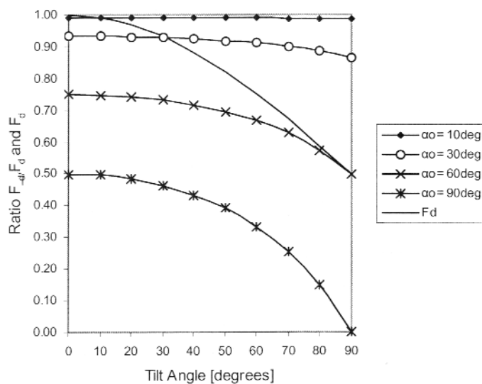
Figure A4: Variation of \hat{F}_d / F_d with \alpha_o and \beta ; and of F_d with \beta
