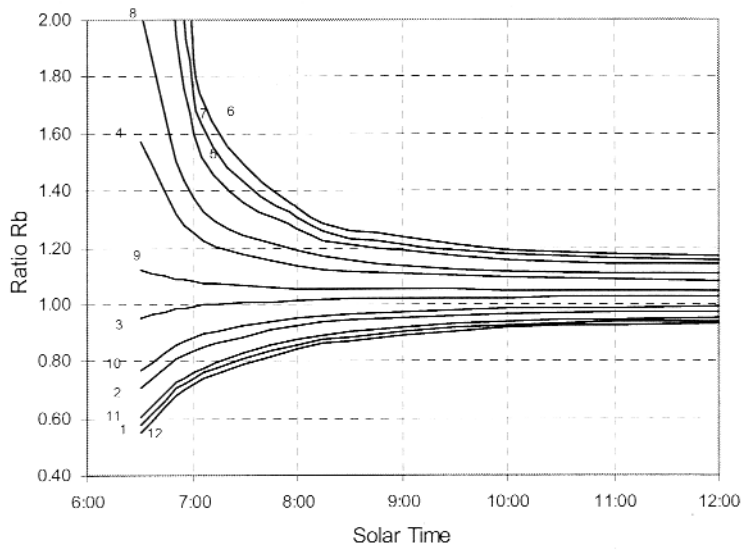
Figure 4a: Ratio R_b for latitude 15^\circ\text{S} for a north-facing collector with tilt angle equal to latitude
